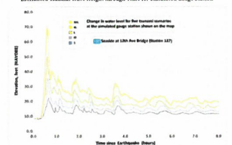
Figure 5: Estimated Tsunami Wave Height through Time for Simulated Gauge Station. A line graph showing the wave height over time for a simulated gauge station.
