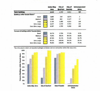
Figure 4: Buildings within Tsunami Inundation Zones. A table and bar chart showing the number and types of buildings within the inundation zones.
