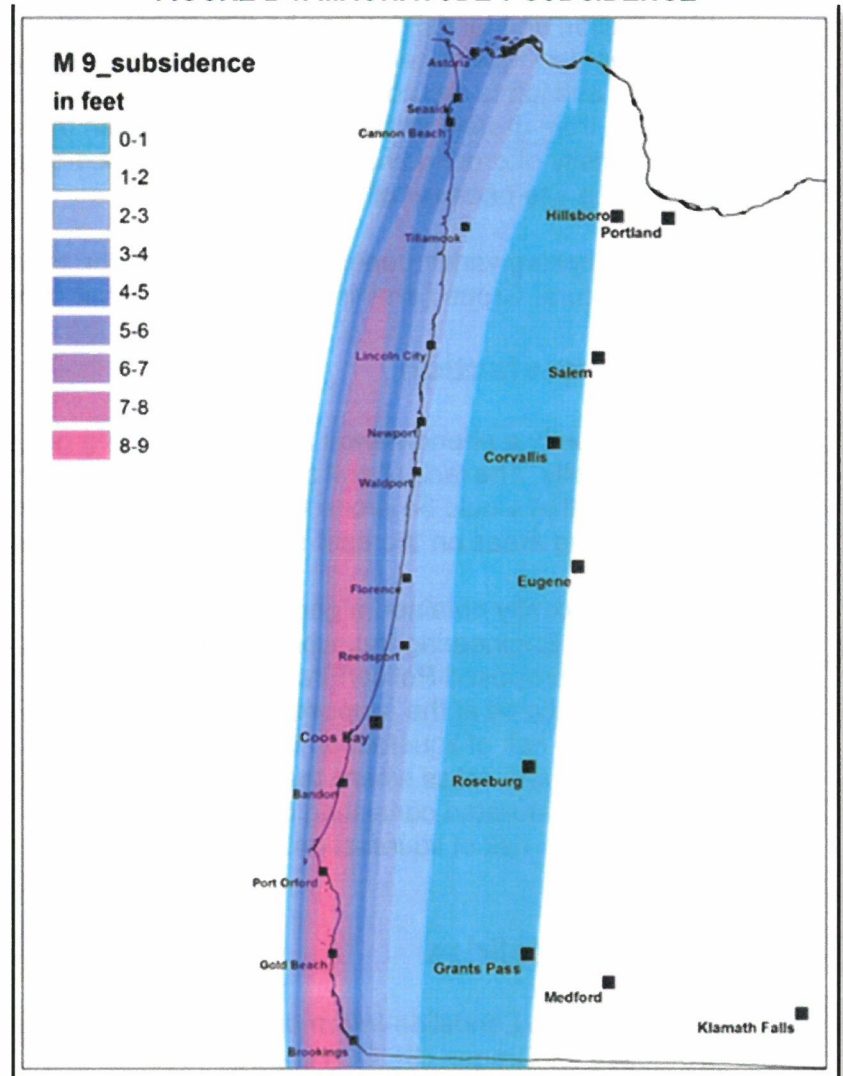
FIGURE 2-4: MAGNITUDE 9 SUBSIDENCE
