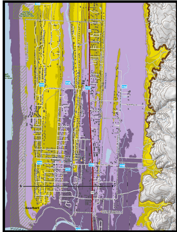
FIGURE 2-1: DOGAMI TSUNAMI INUNDATION MAP
